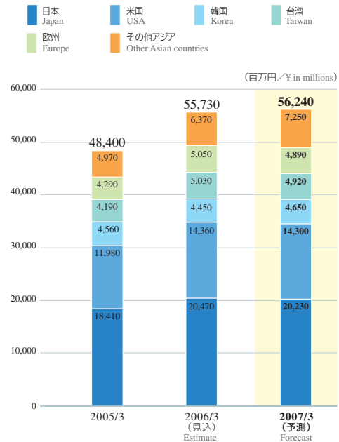
SMIFオープナ/FOUPオープナ販売金額推移 Sales of SMIF opener/FOUP opener
