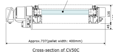
Cross-section of CV50C
